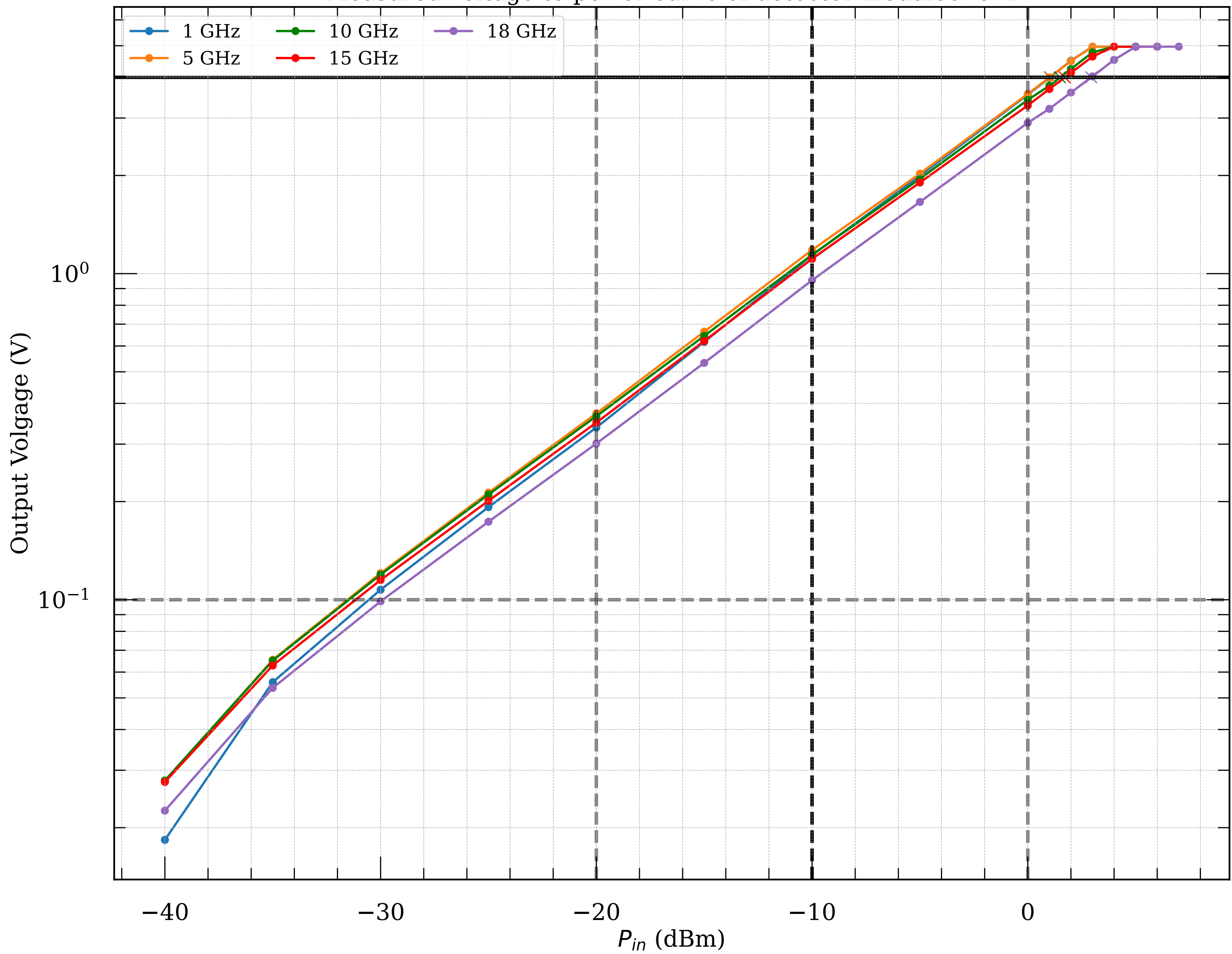
Measured voltage-to-power curve of detector module076v2
